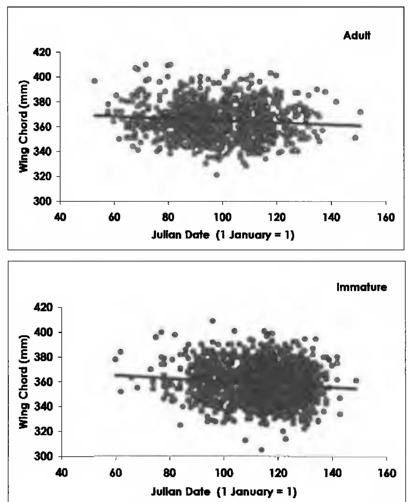
Figure 2. Wing length of adult ( r = -0.083 , P = 0.012 , N = 906 ; regression y = -0.078 (\pm 0.031) - 0.083 ; top) and immature ( r = -0.087 , P < 0.003 , N = 1709 ; regression y = -0.108 (\pm 0.030) - 0.087 ; bottom) buzzards in relation to date of passage and trapping at Elat.
